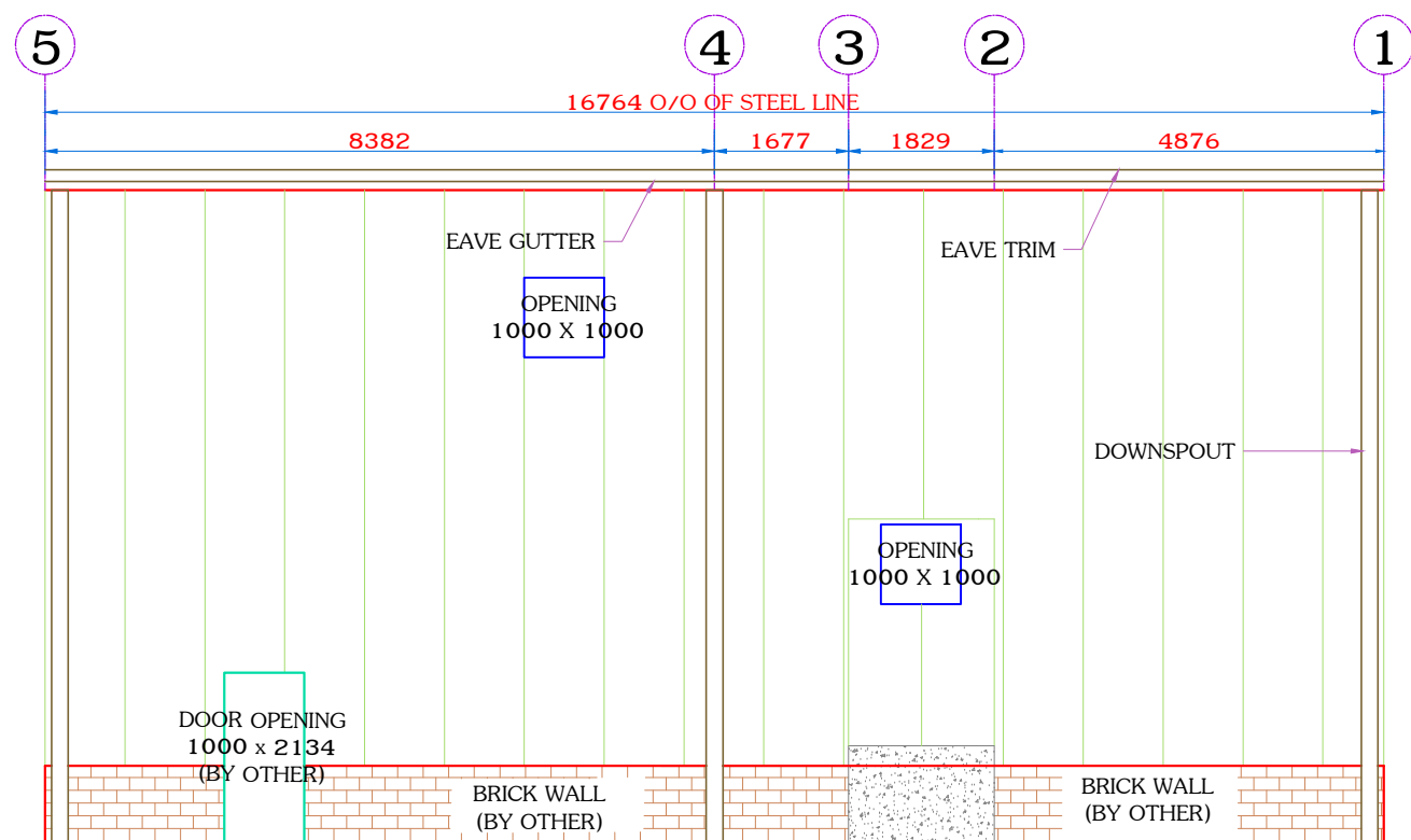
SIDE WALL SHEETING @ GRID-A
