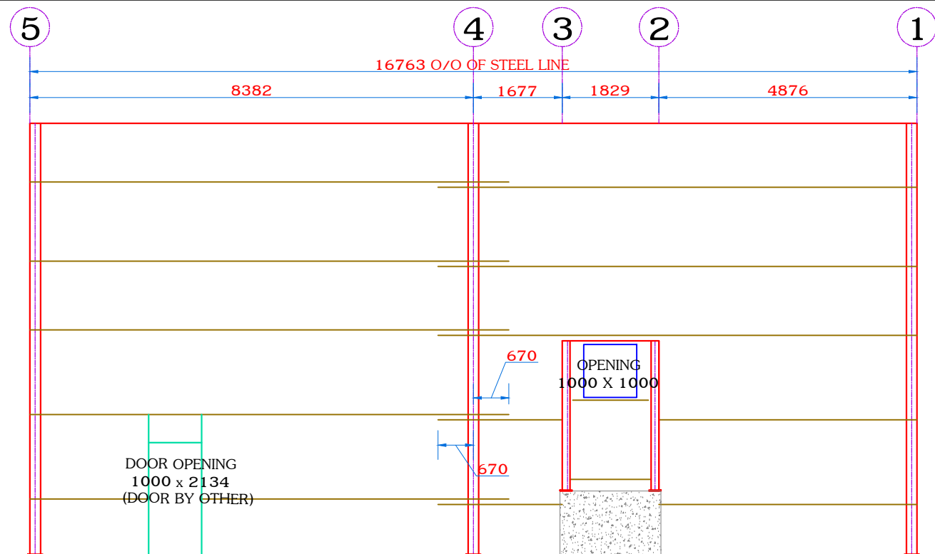
SIDE WALL FRAMING @ GRID-A
